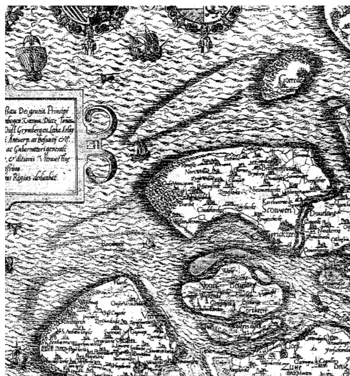
fig. 27 The estuarine branches extended far into the North Sea. At the coast there was an extensive area of gullies and sandbanks. In this figure, the situation in 1560 is shown as presented by Jacob van Deventer.
